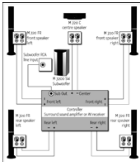
Figure: Audio connection diagram
